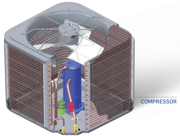
COMFORT™ 16 AIR CONDITIONER
